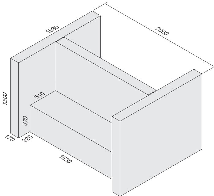
MS DOUBLE TWIN 2000/1630
