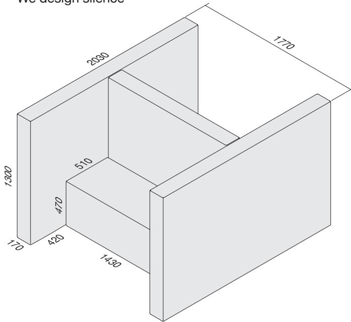
MS DOUBLE TWIN 1600/2030
