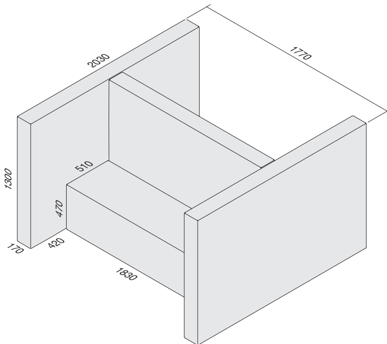
MS DOUBLE TWIN 2000/2030
