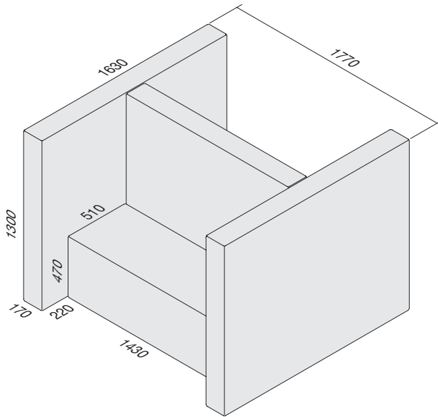
MS DOUBLE TWIN 1600/1630
